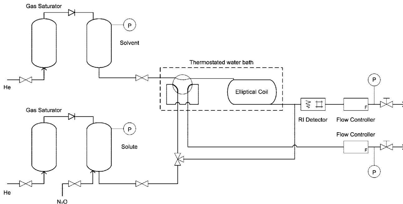
Figure 1. Schematic representation of the Taylor dispersion setup.
