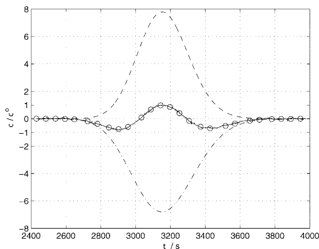
Figure 3. Typical result from an N_2O + (PZ + H_2O ) system: —, exptl result; \bullet\circ\bullet\circ , fit; --, N_2O response; - · - ·, PZ response.
